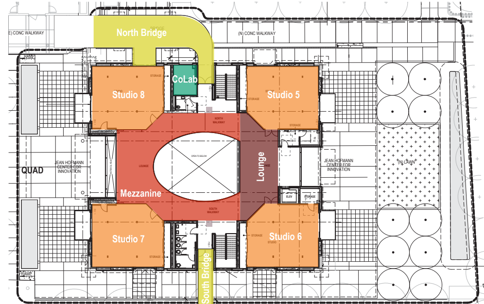
SECOND FLOOR
